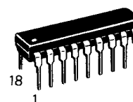
P SUFFIX PLASTIC PACKAGE CASE 707
